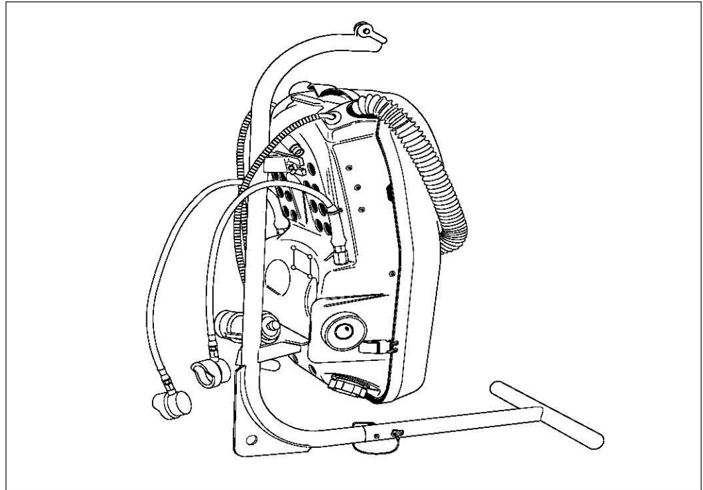
Figure 18-3. Emergency Breathing System.
