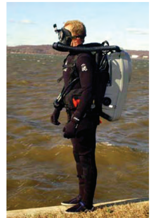
Figure 18-1. MK 16 MOD 1 Closed-Circuit Mixed-Gas UBA.
